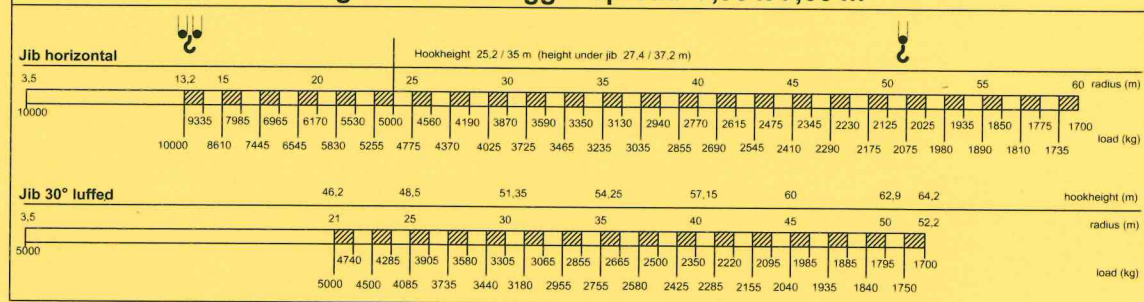
Lifting chart Outrigger spread 7,95 x 5,72 m
